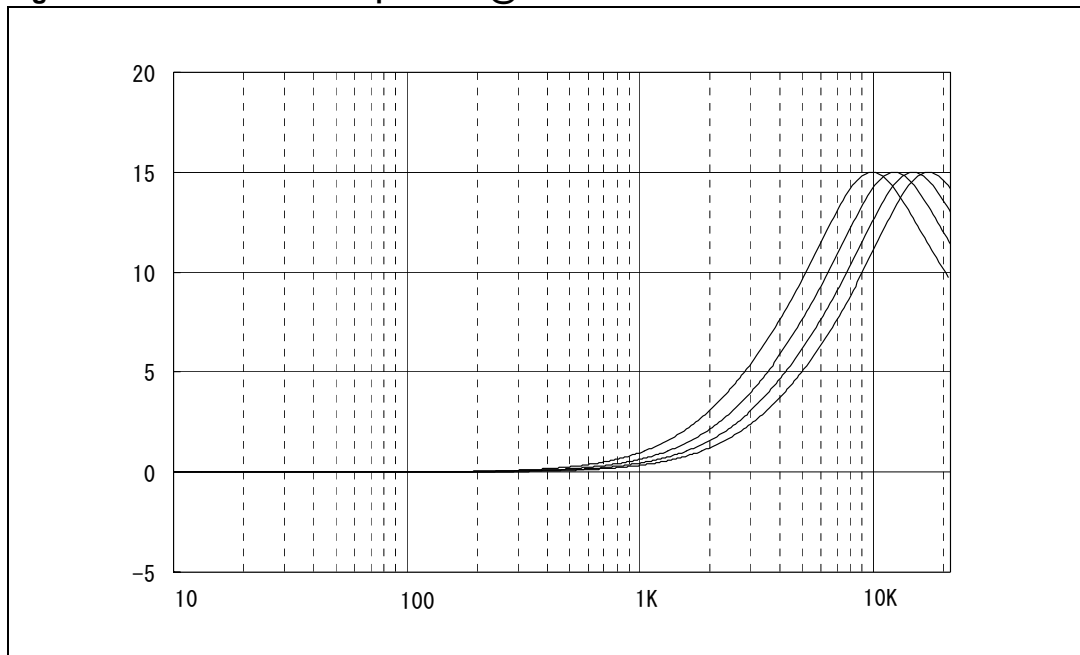
Figure 15. Treble center frequencies @ Gain = 15 dB
